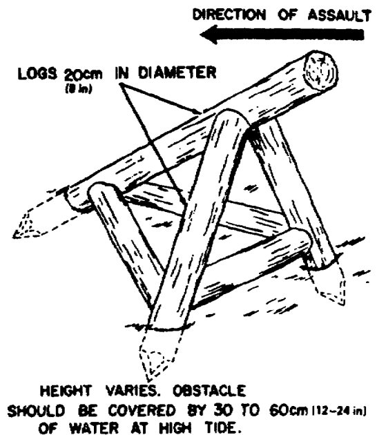
Figure 3-26. Log tripod.
